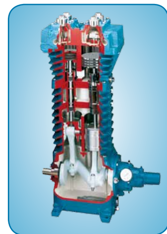
Blackmer HD Series heavy-duty, oil-free, reciprocating gas compressors.
