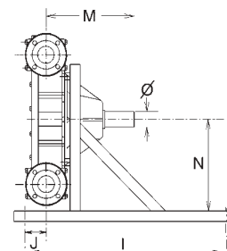
Construction AS (arbre nu)
